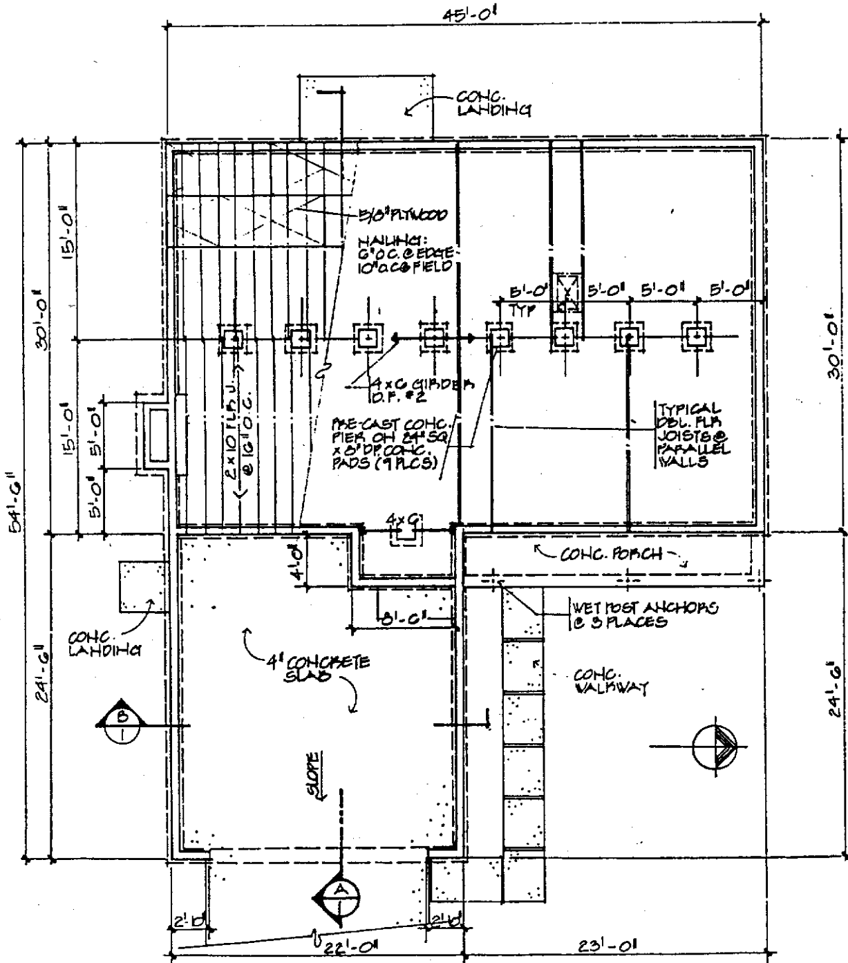
FOUNDATION PLAN
