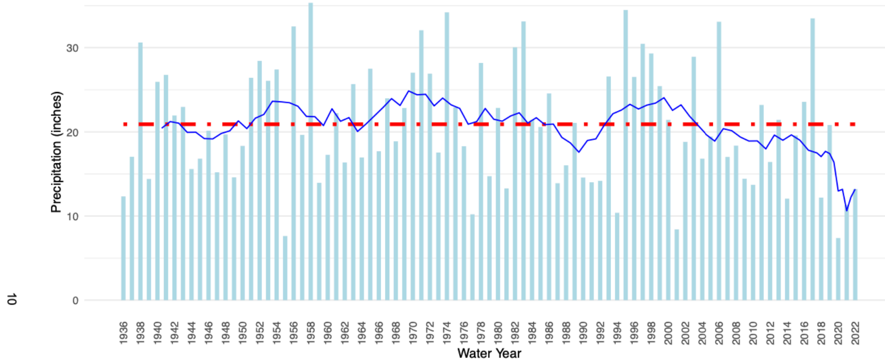
Figure 4: Fort Jones annual precipitation from 1935 to 2022, according to CDEC data. The long term mean is shown as a red dashed line, and the ten year rolling mean is the blue trendline.
